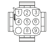
CHASSIS HARNESS CONNECTOR (C1) (MATING SIDE)
