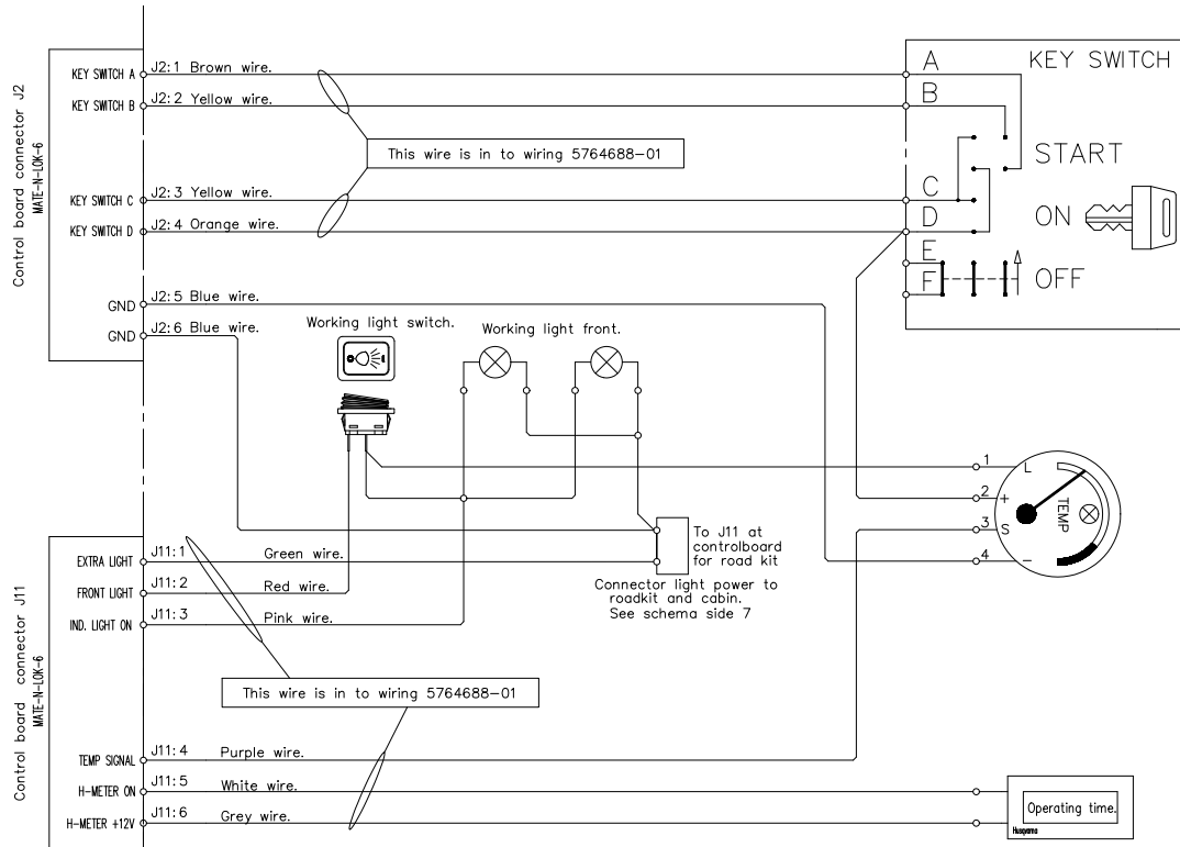
P520 D Schema side 3 Control board 576 97 50-01
