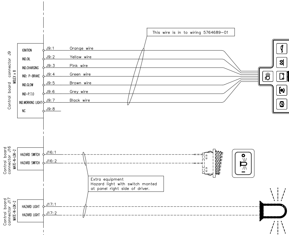
P520 D Schema side 5 Control board 576 97 50-01
