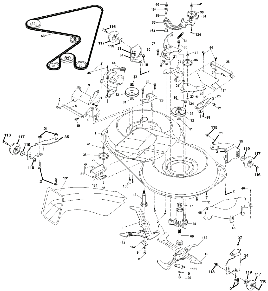
107cm_deck-elect(CRD)_3
