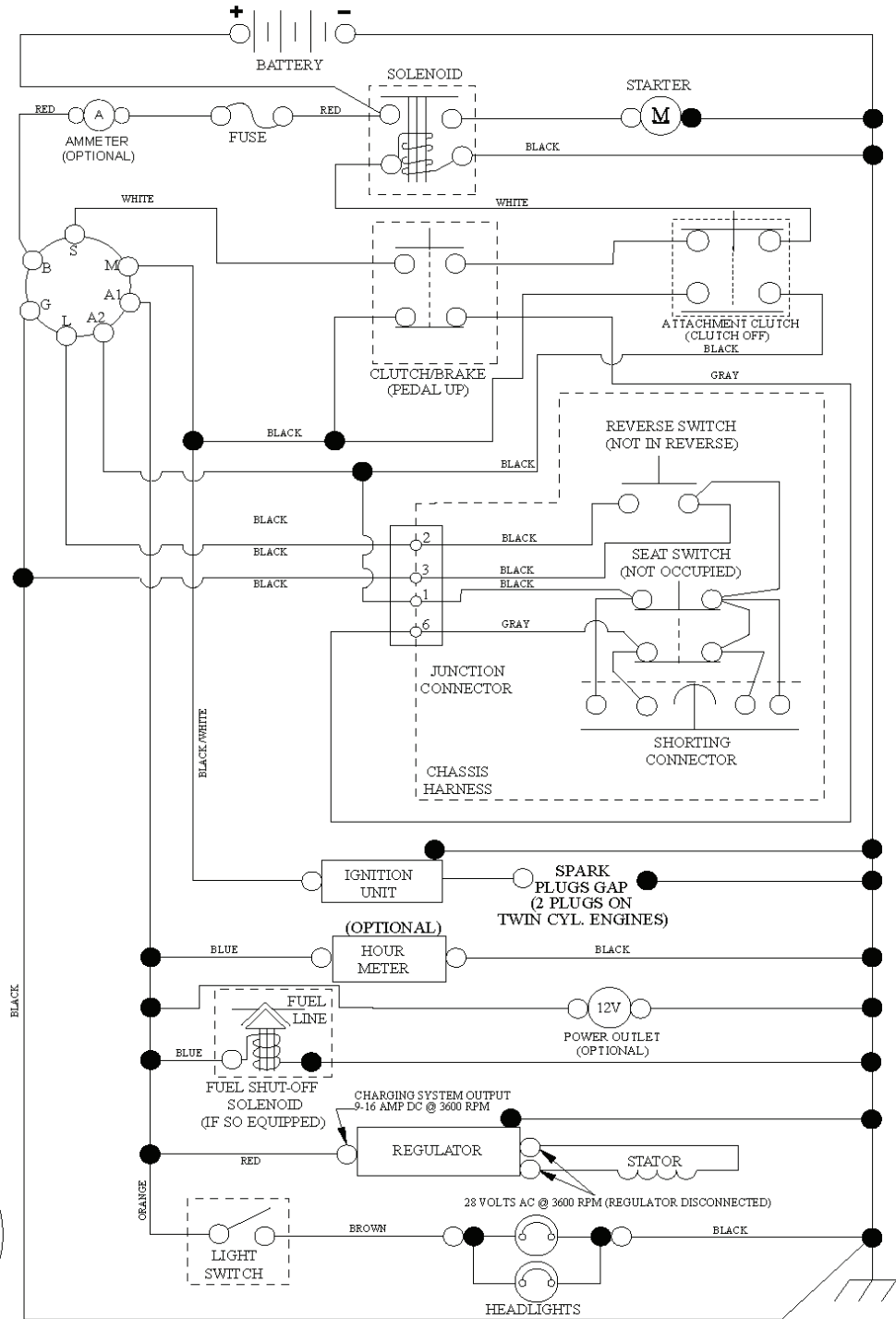
NON-REMOVABLE CONNECTIONS
